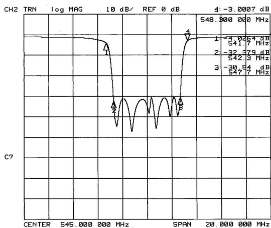
Typical Frequency Response of 3271ABU
