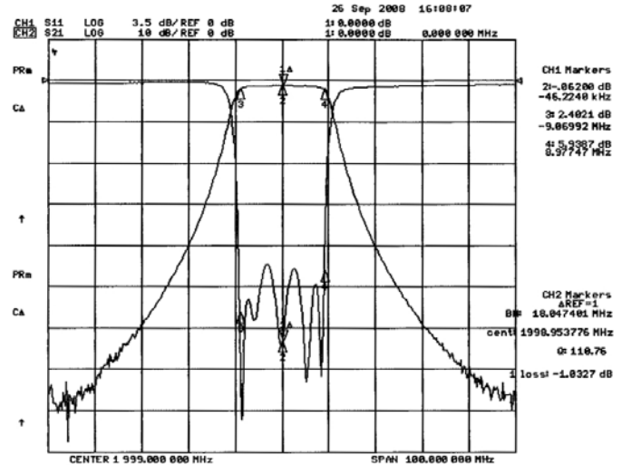
Typical Frequency Response of 5948
