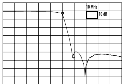
Typical Frequency Response of 5KLP
