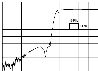
Typical Frequency Response of 5KHP
